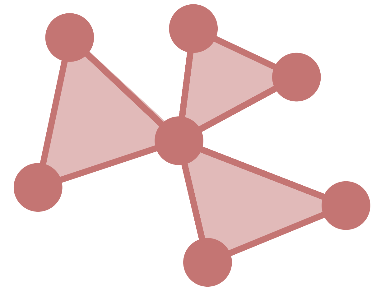
Second order hubs
