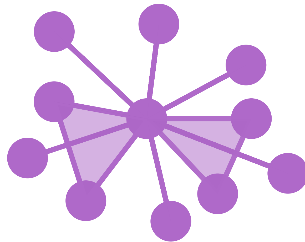
Pairwise and second order hubs
